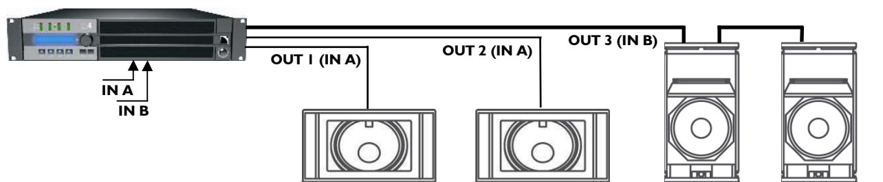
Figure 13: Two SBI 18 and two ARCS ® connected to an LA4 controller
