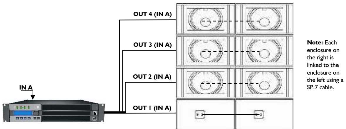
Figure 12: Two basic SBI 18 cardioid arrays connected in parallel to an LA8
