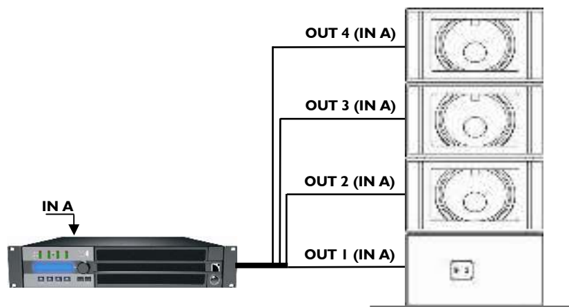
Figure 11: One basic SBI 18 cardioid arrays connected to an LA4
