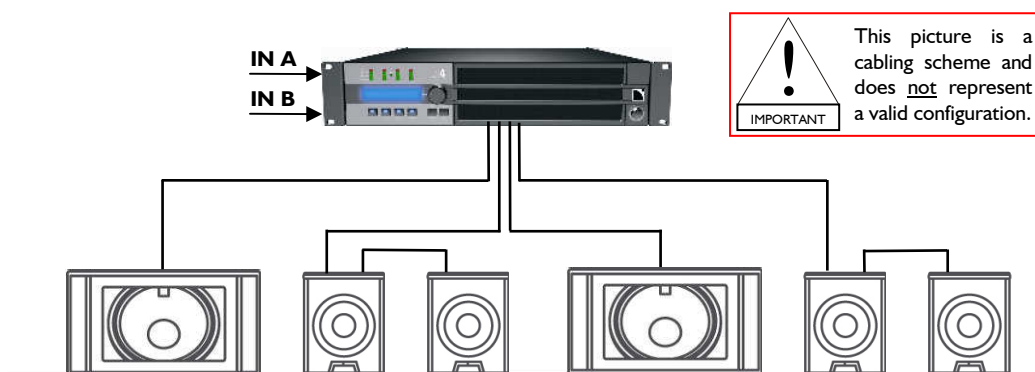
Figure 6: Four 8XTi and two SB18i enclosures connected to an LA4 / LA4X controller
