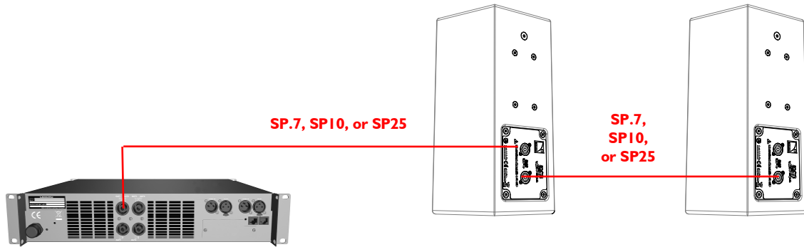
Figure 3: Connecting two 8XTi in parallel to the LA4 / LA4X amp channel #1
