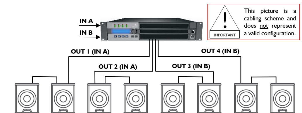
Figure 5: Eight 8XTi enclosures connected to an LA4 / LA4X controller
