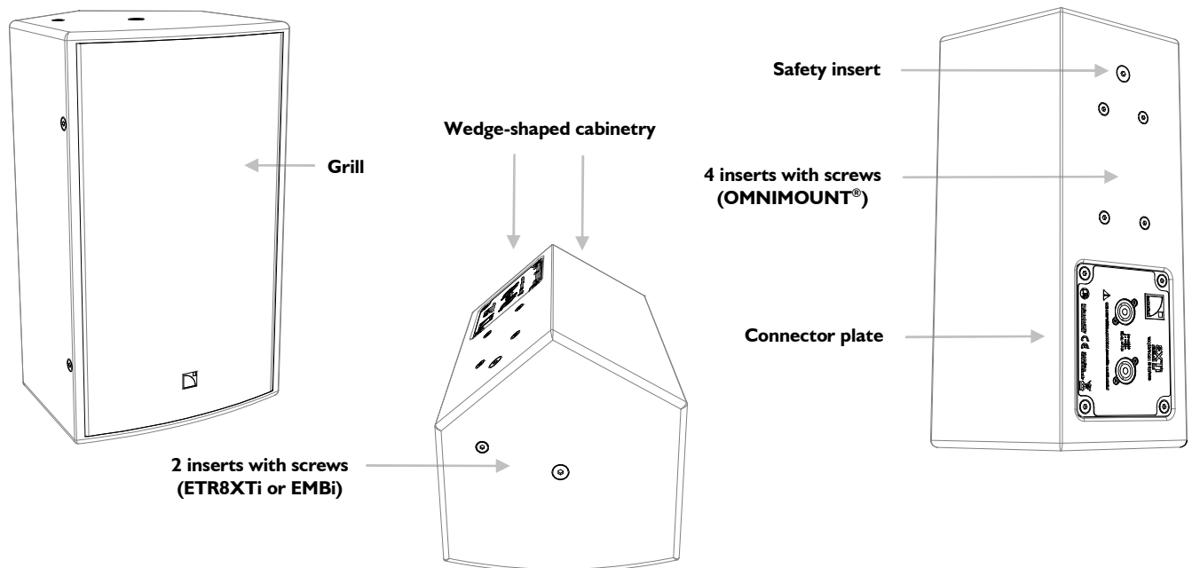
Figure 2: The 8XTi enclosure
