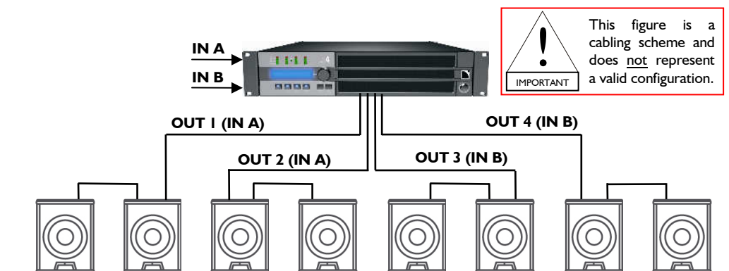
Figure 4: Eight 8XTi enclosures connected to an LA4 / LA4X controller
